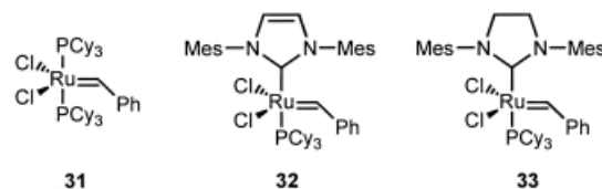
Figure 1. Ruthenium catalysts.
